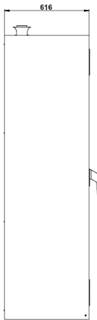
Side view G90.205.060.2F
