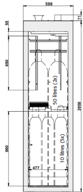
Sectional view G90.205.060.2F
